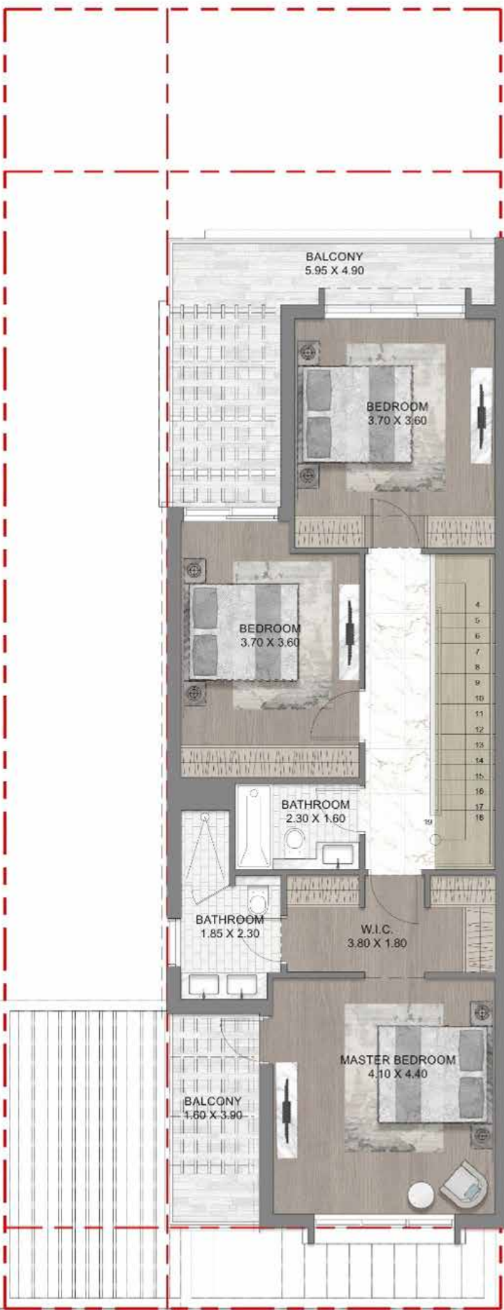
FIRST FLOOR
